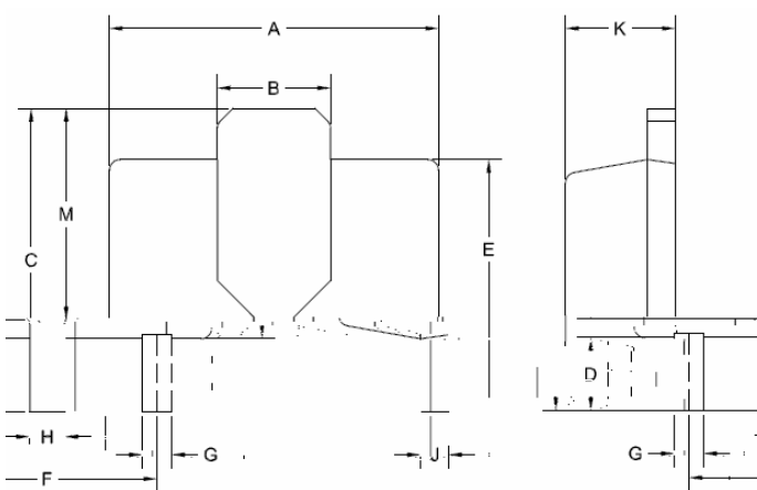
TOM VIEW
