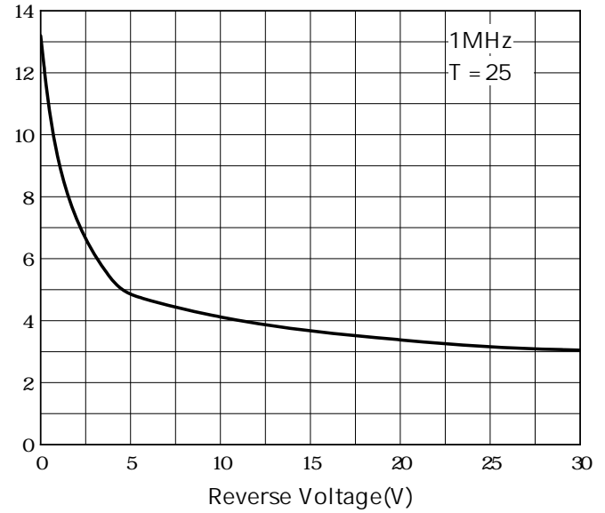
Fig.2: Capacitance Characteristics
