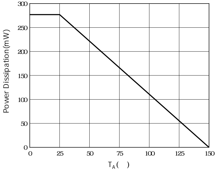
Fig.15 P_D - T_A
